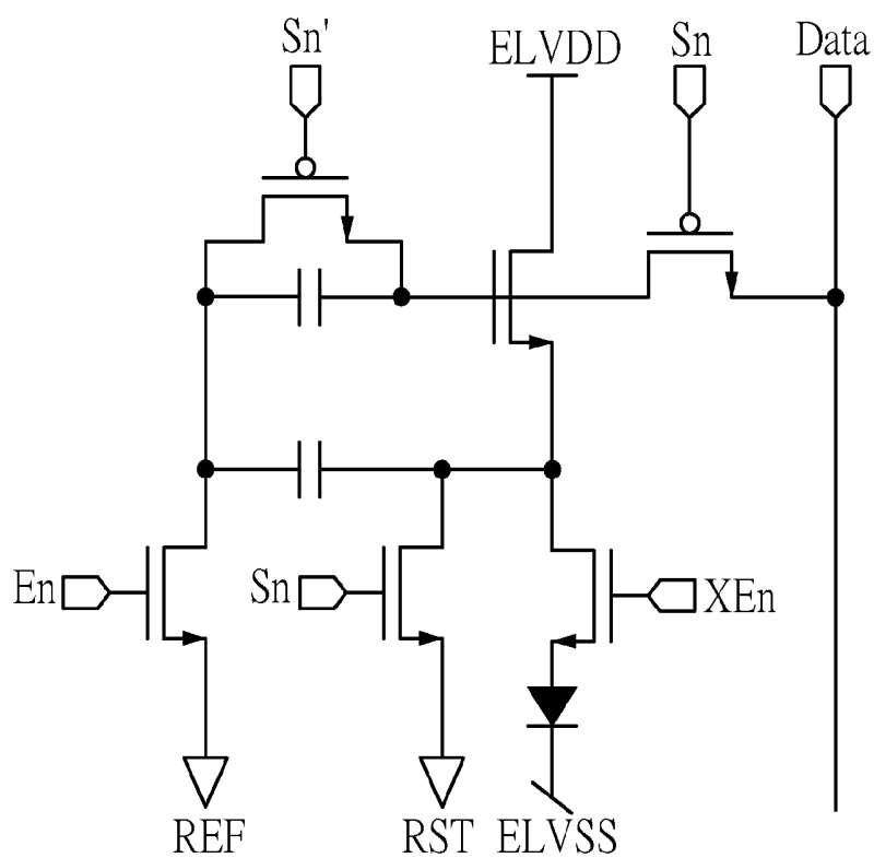
FIG. 3(PRIOR ART)
